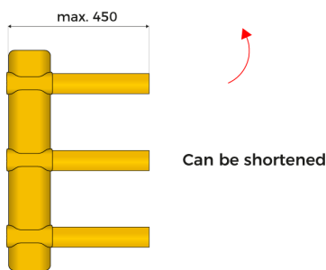
Expansion modules for Universal protector 700
