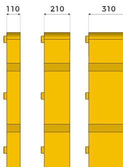
Expansion modules for CP200
